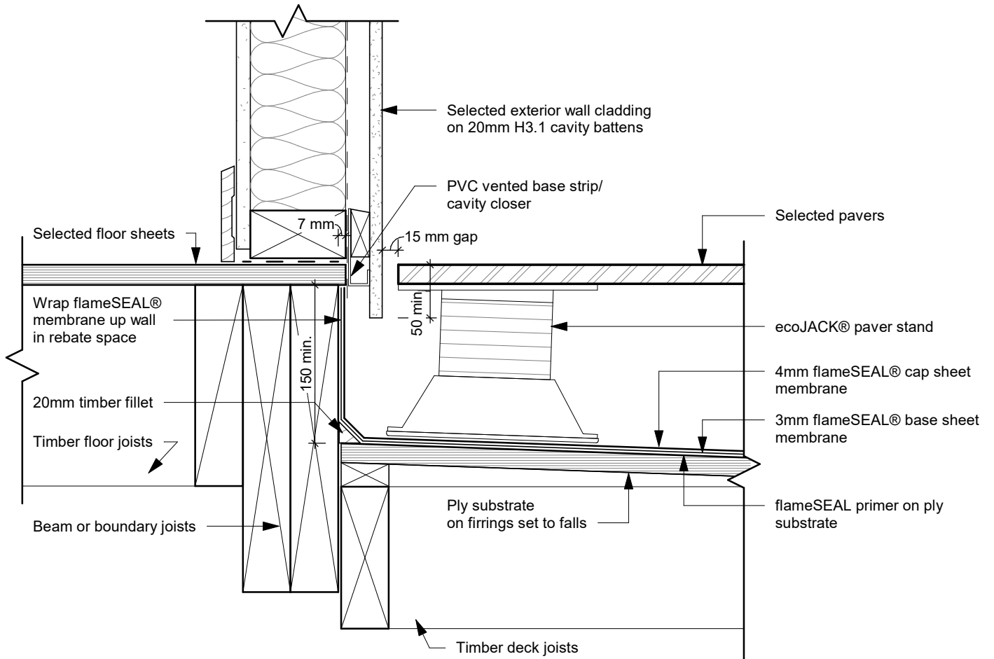
fS D32 - ecoJACK® Paver - Wall Detail - Type 2
