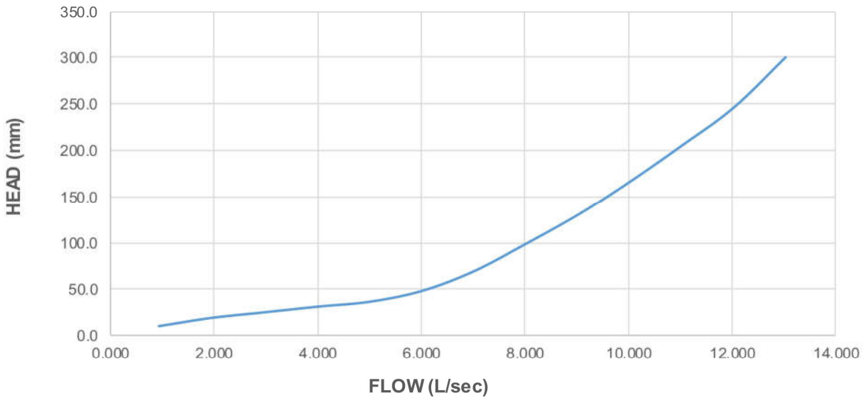
Flow Characteristic Curve for: Roof Drain 100mm Condition: Fitting only
