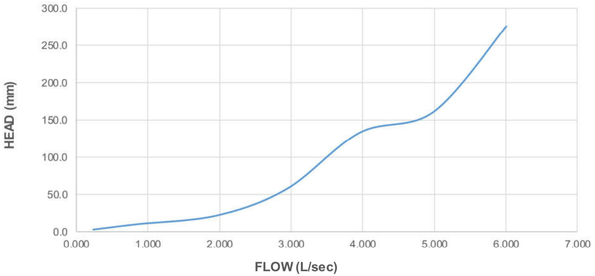
Flow Characteristic Curve for: Roof Drain 65mm Condition: Fitting only
