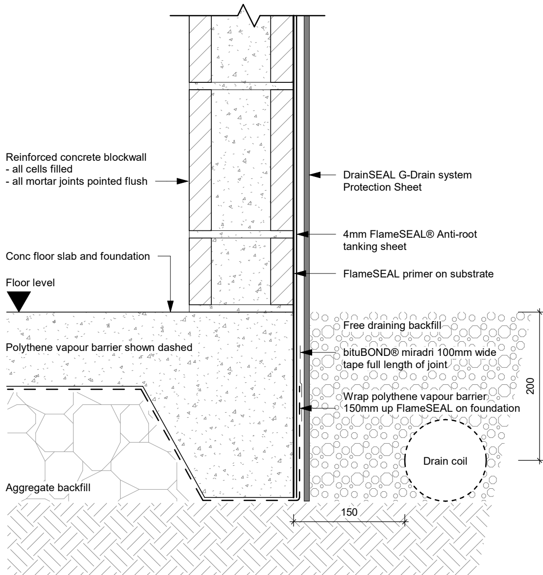
fS-T21 - Blockwall/ Floor Joint 1-2 (Single Layer)
