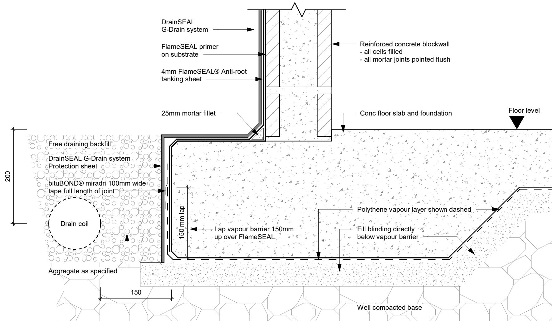
fs-T D20 - Blockwall/ Floor Joint 1-1 (Single Layer)
