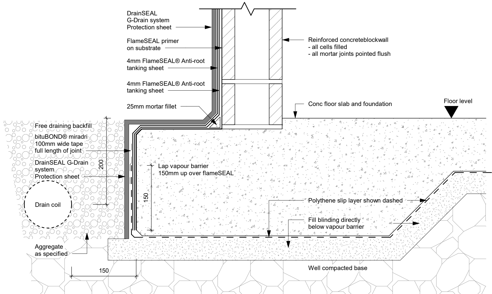
fS-T D13 - Blockwall/ Floor Joint 2-2 (Two Layer)
