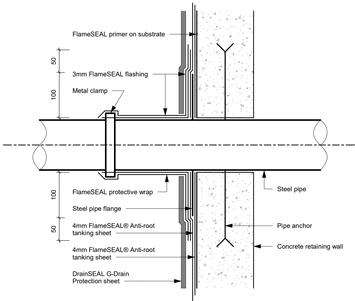
fS-T D03 - Concrete/ Pipe Penetration (Two Layer)
