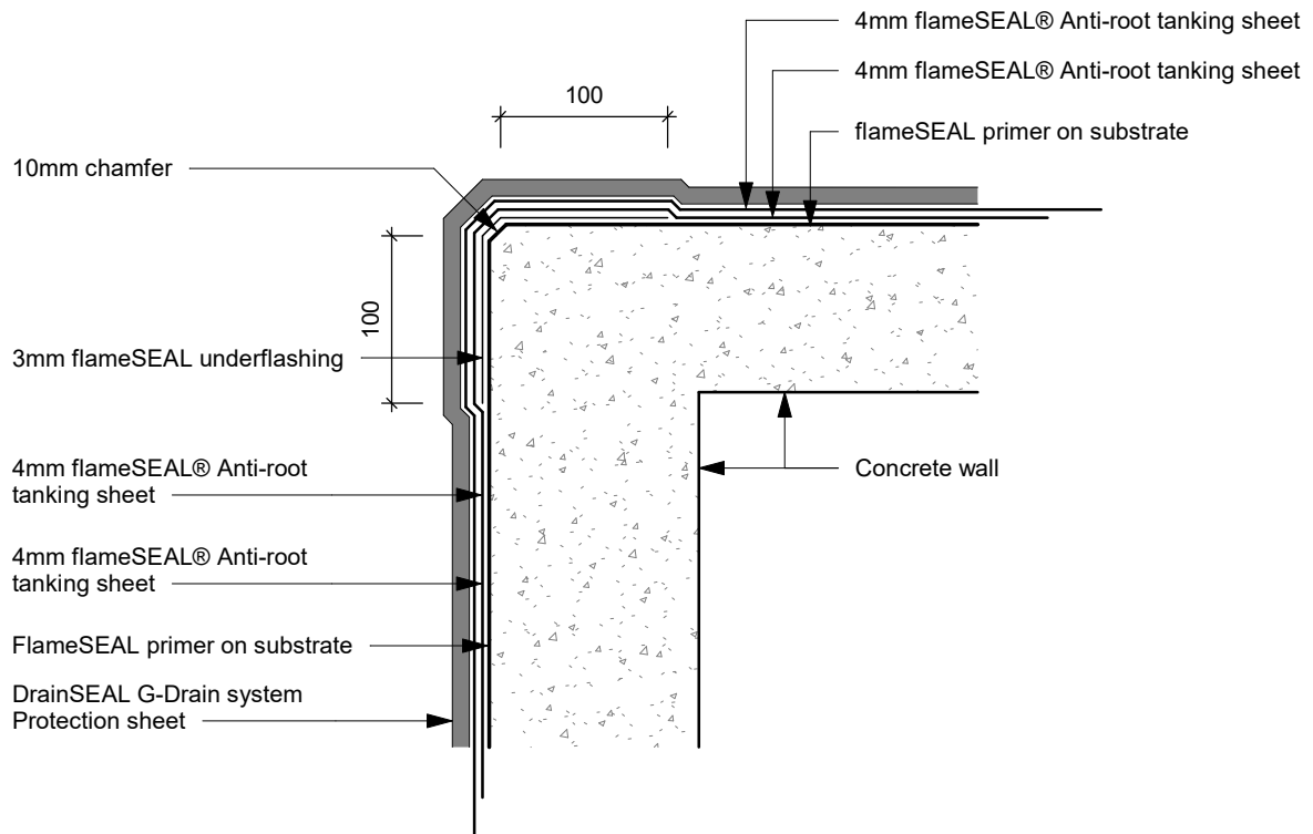
fS-T D02 - Exterior Concrete Corner (Two Layer)
