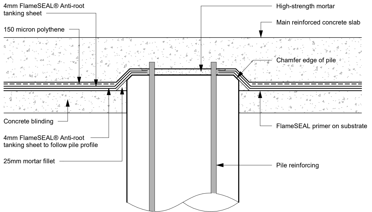
fS-T D07 - Pile Cap Detail (Two Layer)
