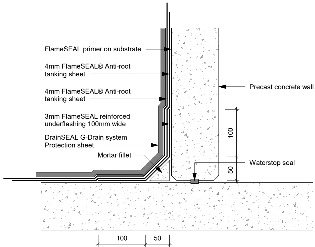
fS-T D17 - Wall T-Junction - Plan (Two Layer)
