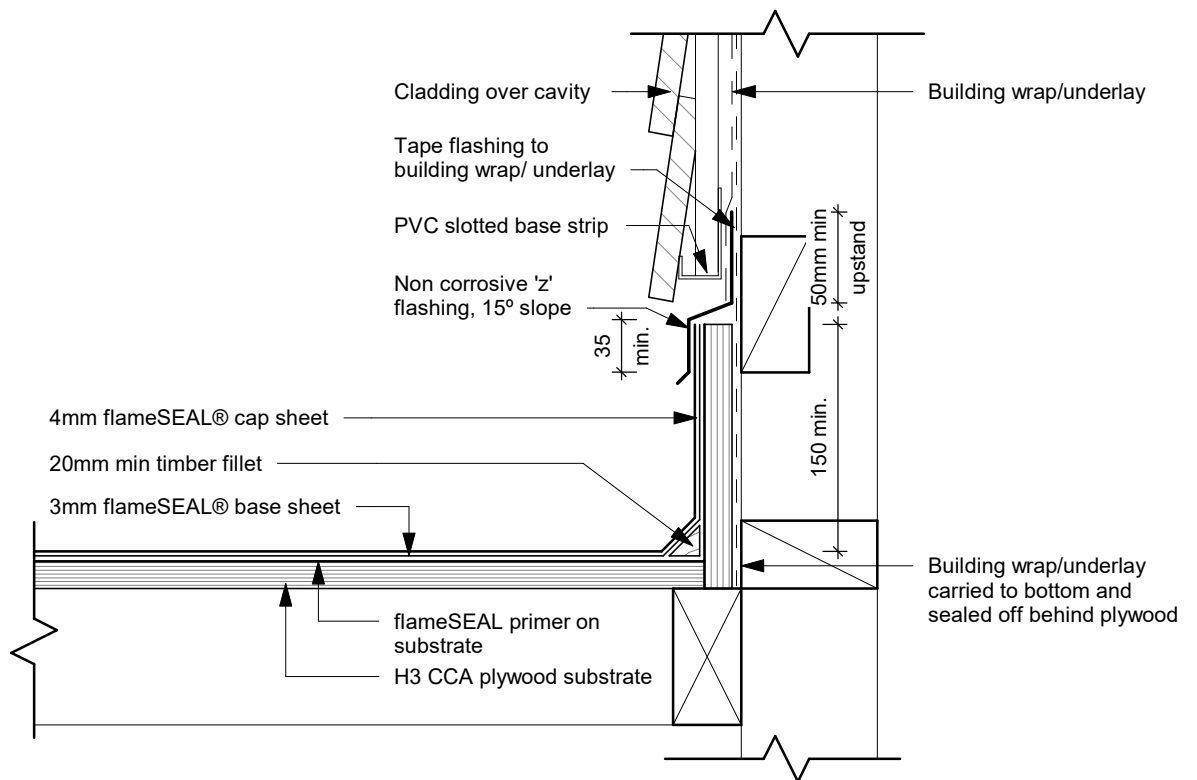
fS D16 - Gutter Upstand - Cladding over Cavity Type 2
