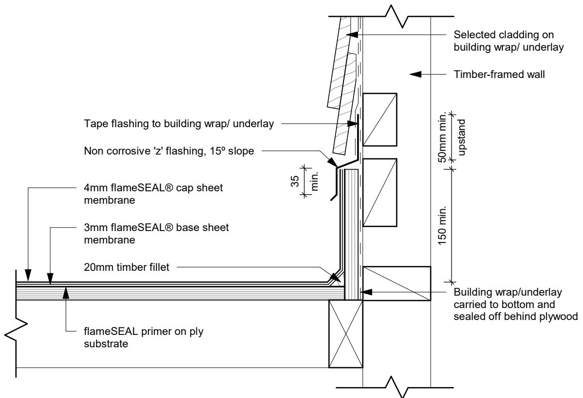
fS D14 - Gutter Upstand 2 - Direct-Fixed Cladding
