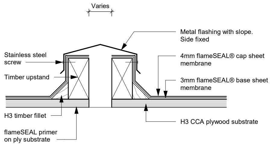
fS D03 - Roof expansion cap detail
