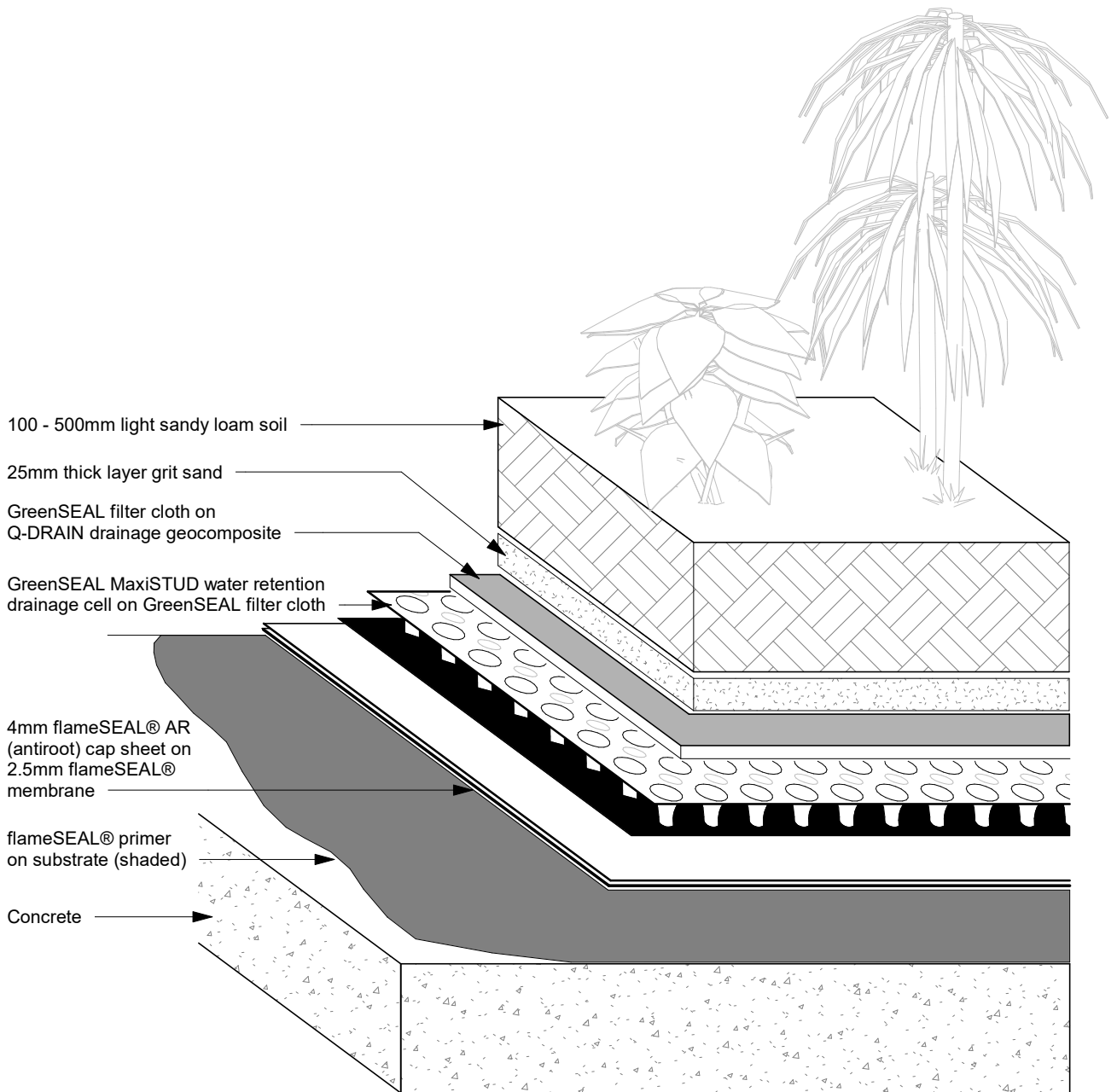
GS D09 GreenSEAL (fS-AR)™ 3D Cutaway
