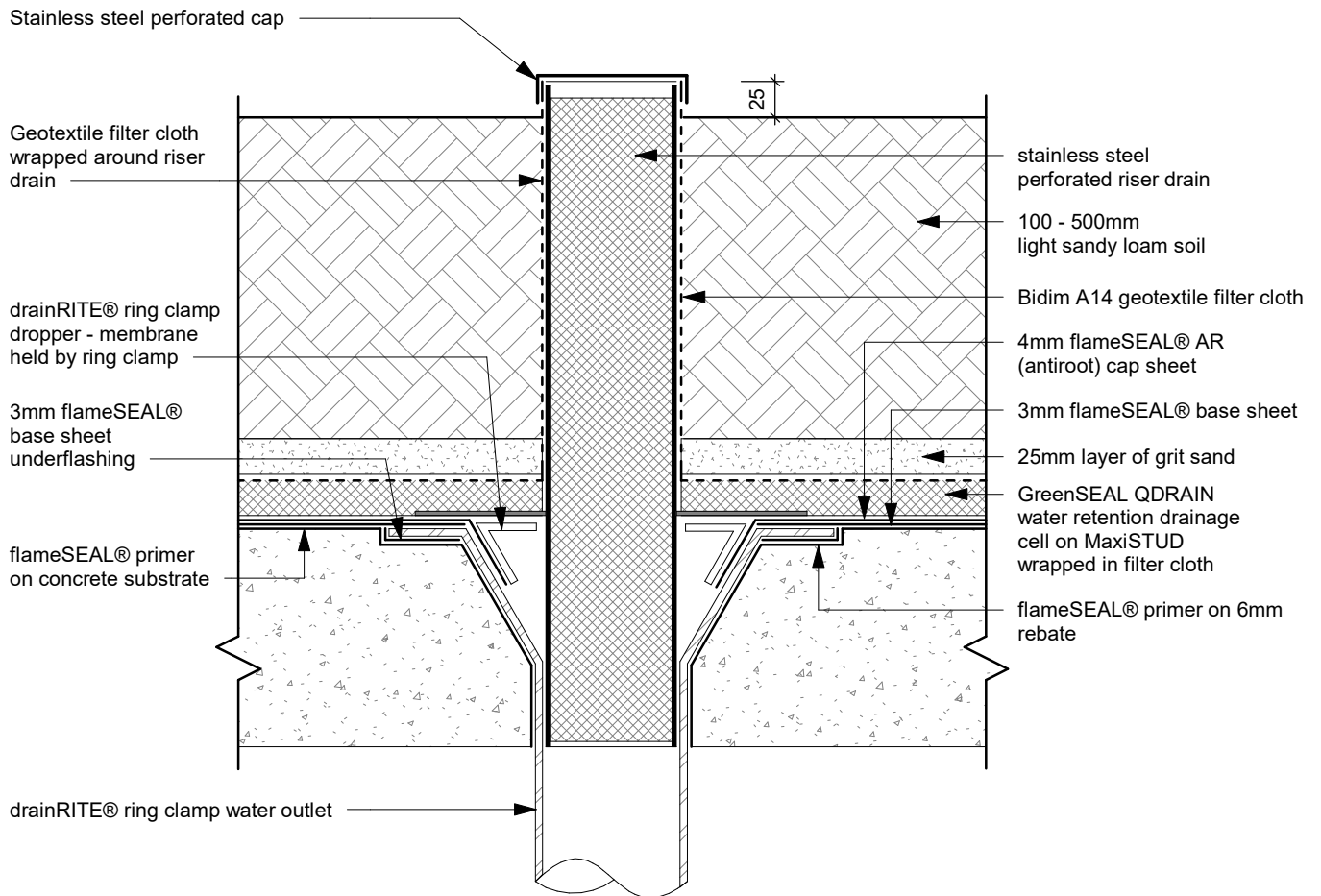
GS D07 (fS-AR) - Soil drainRITE® Outlet
