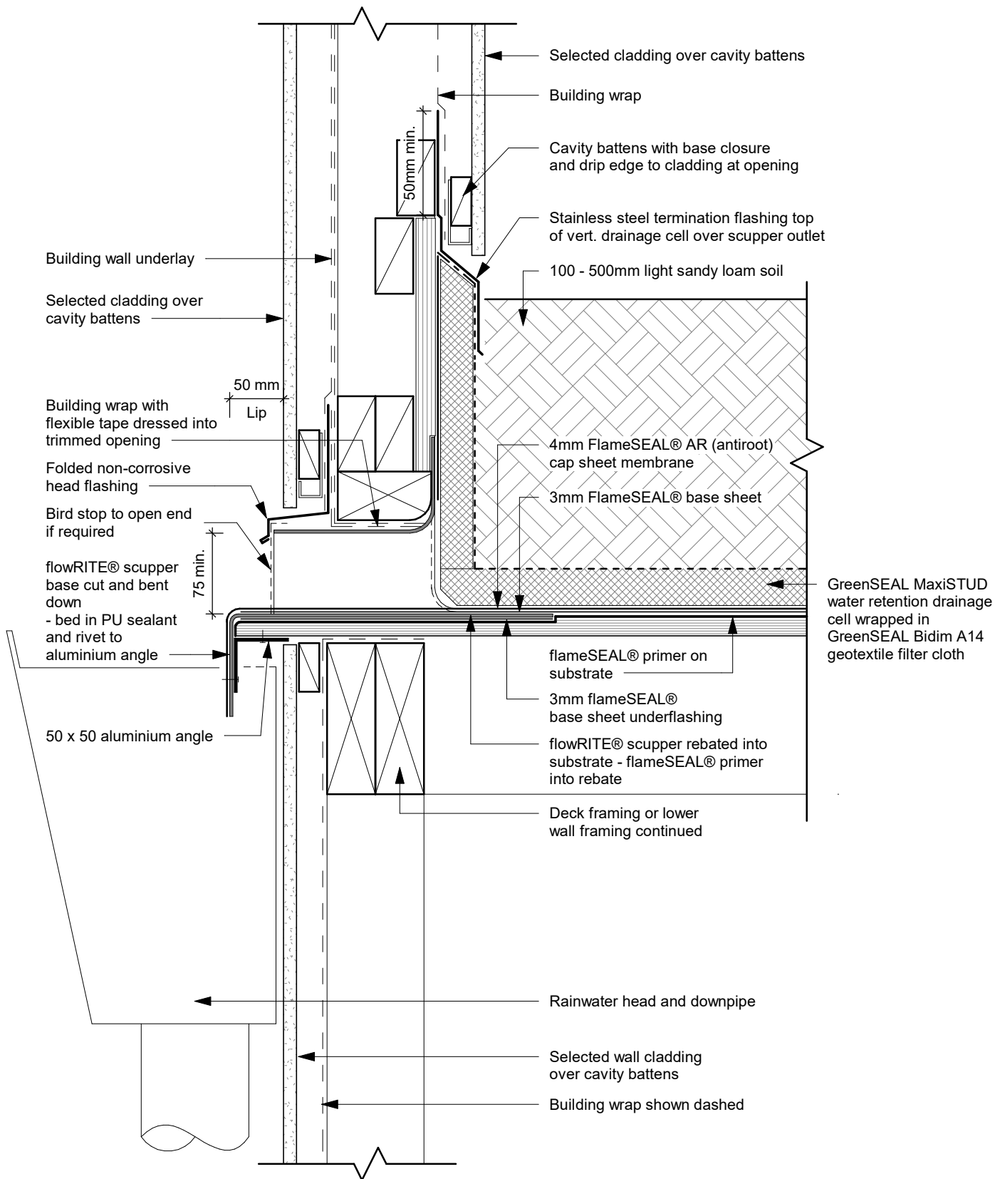
GS D08 - (fS-AR) Soil flowRITE® Scupper
