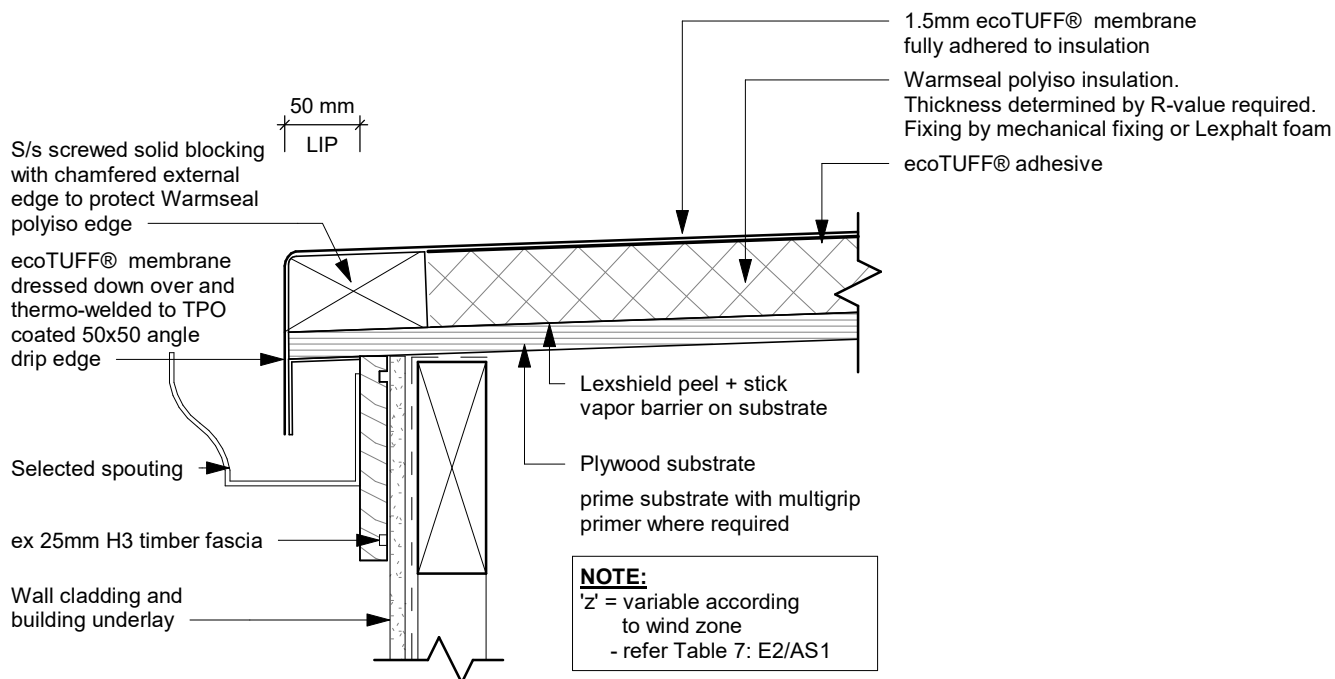
WS ET005 - External Gutter - Type 2 Revision: 28 June 2019
