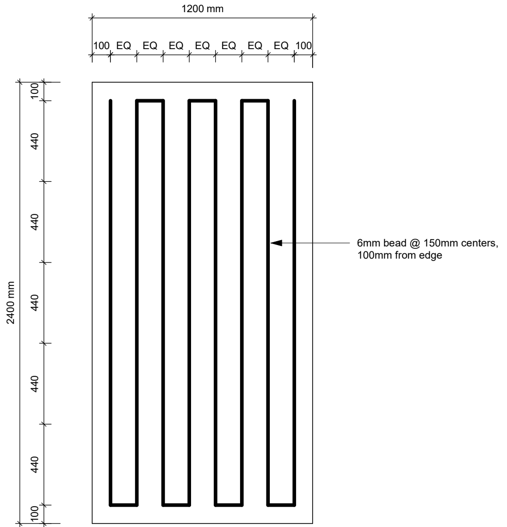
WS ET003 Lexphalt Adhered Warmseal Polyiso Boards
