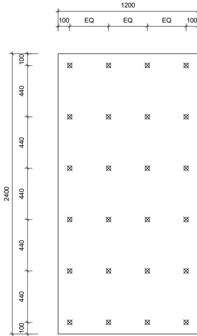
WS ET002 Mechanically fixed Warmseal Polysio
