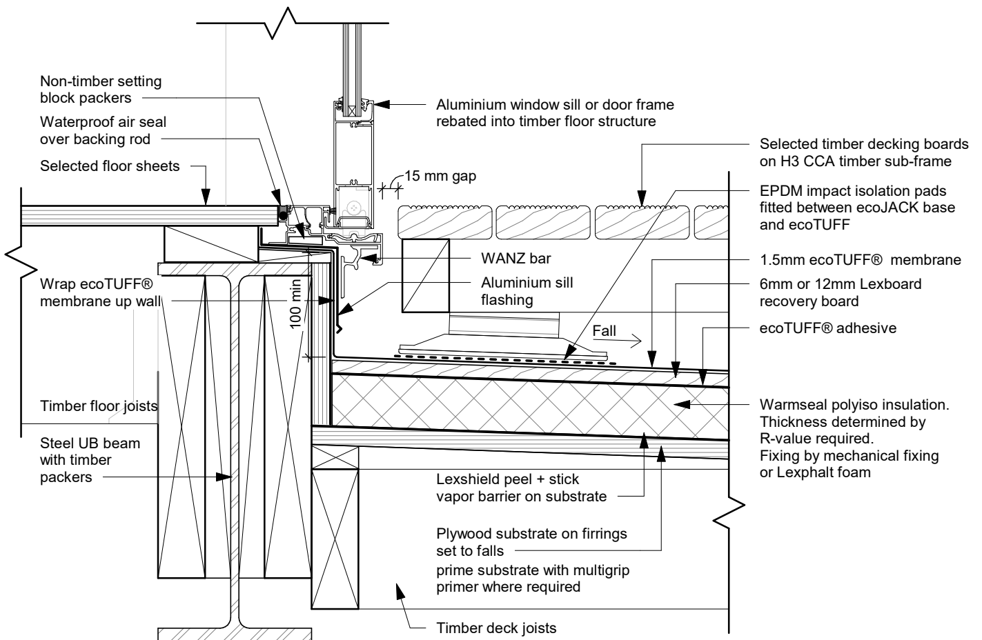
WS ET036 - timber raft floating deck - threshold detail - type 2
