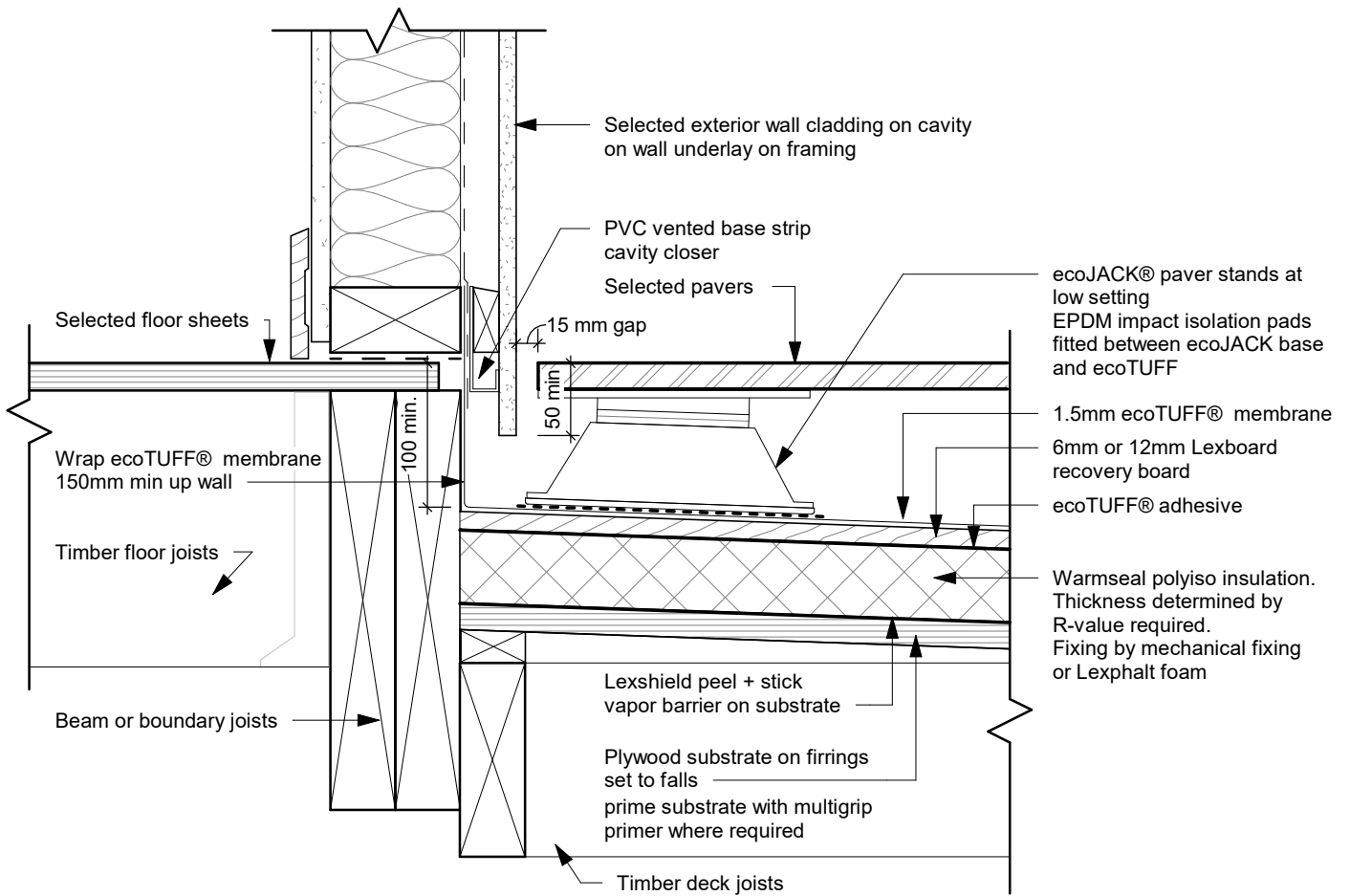
WS ET030 - ecoJACK® Paver - Wall Detail - Type 1
