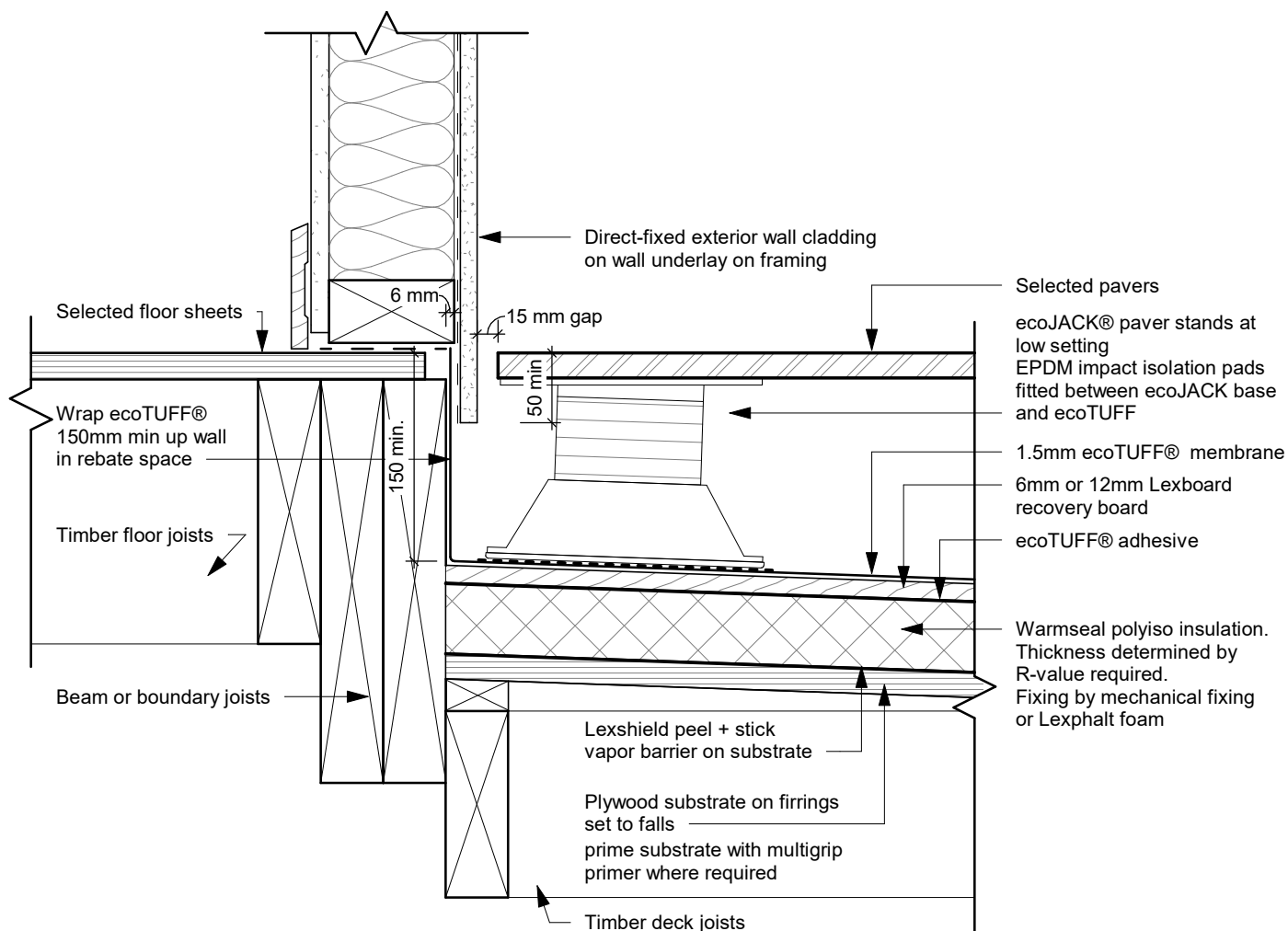
WS ET031 - ecoJACK® Paver - Wall Detail - Type 2
