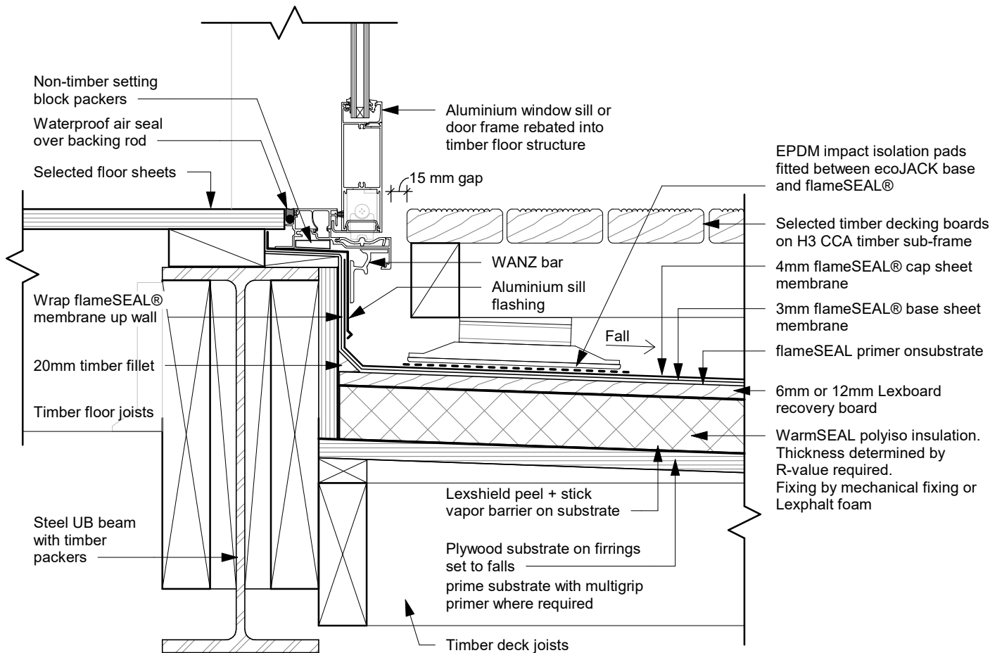
WR fS D36 - timber raft floating deck - threshold detail - type 2
