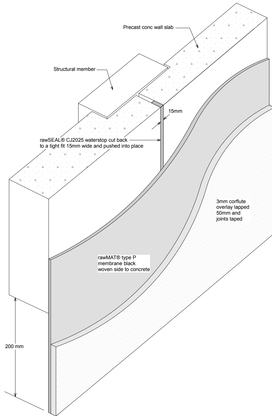
b-RAW15 - Panel to Panel Iso View
